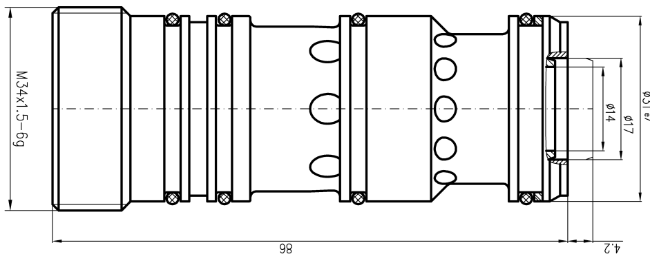
Technical drawing of the pm3/val/dn20/a valve cartridge
