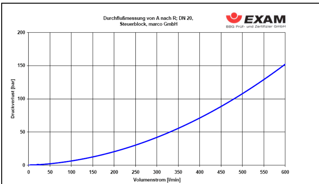
Flow rate measurement of the pm3/val/dn20/a valve cartridge
