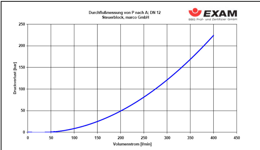
Flow rate measurement of the pm3/val/dn12/a valve cartridge
