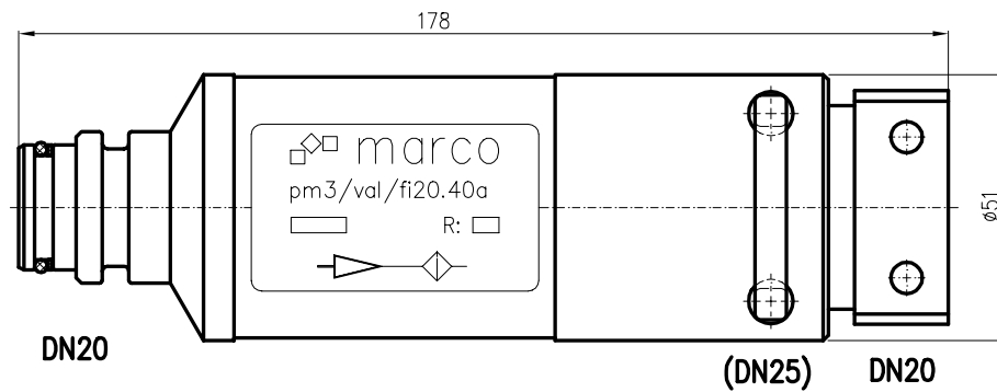
Picture: pm3/val/fi.. In-line filter DN20
