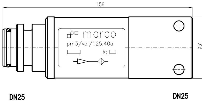
Picture: pm3/val/fi.. In-line filter DN25
