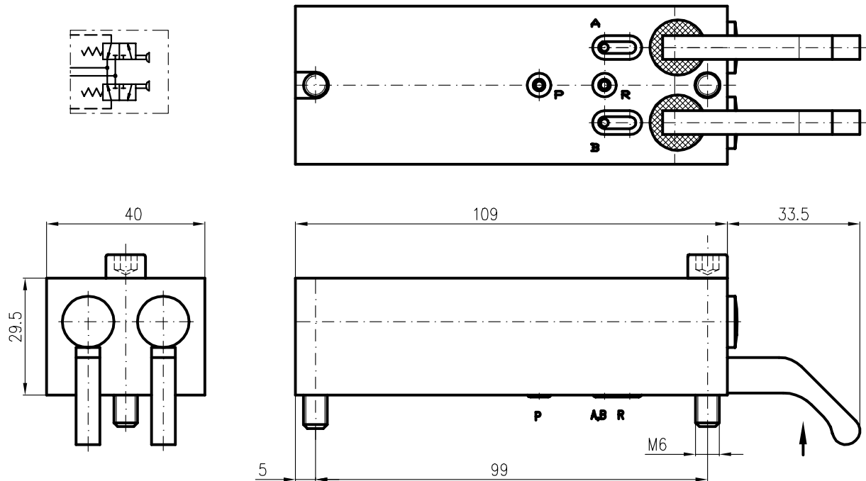
Picture: pm3/val/evv/h1 Manual pilot valve
