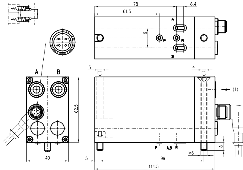
Picture: pm3/val/evv/a.. Double solenoid pilot valve
